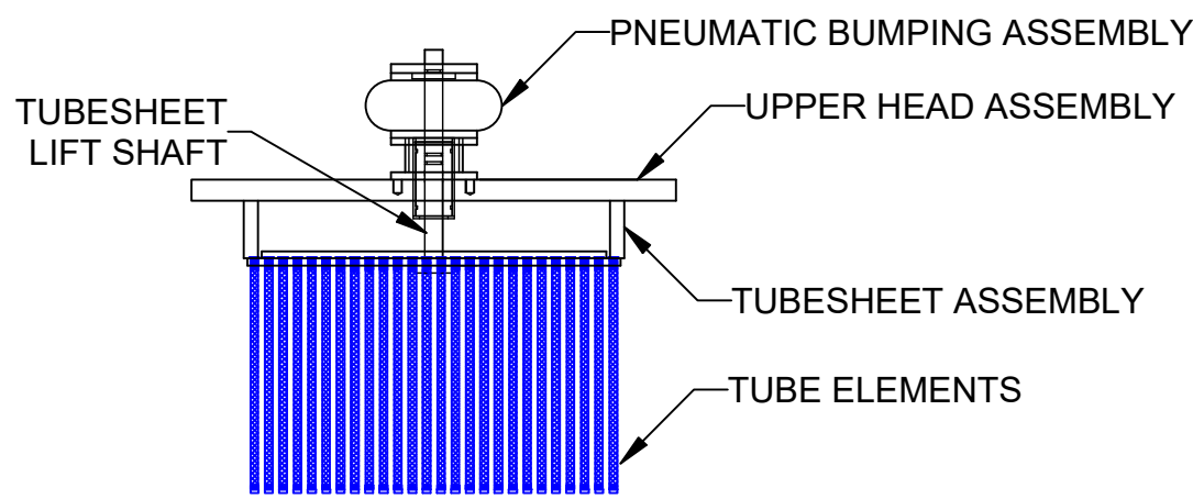
UPPER HEAD AND ELEMENT DETAIL
